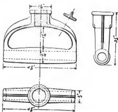
Fig. 3241. Handle for Sandbox Rod.
